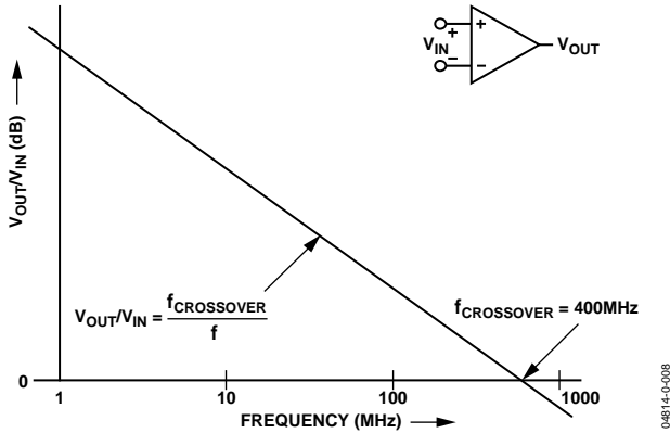
Figure 63. Open-Loop Response
