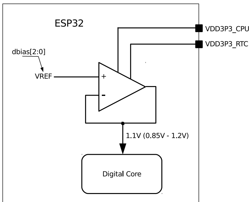
Figure 152: Digital Core Voltage Regulator
