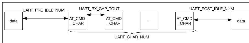
Figure 71: AT_CMD Character Format
