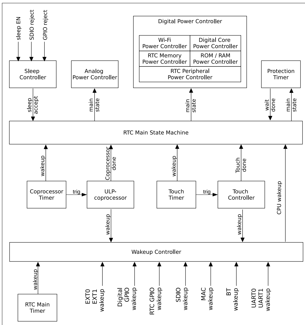
Figure 156: RTC Structure
