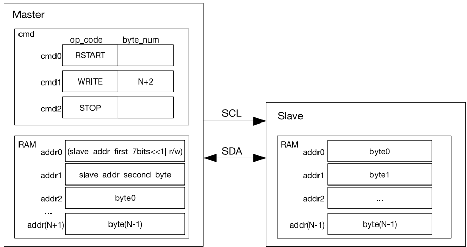
Figure 42: I2C Master Writes to Slave with 10-bit Address
