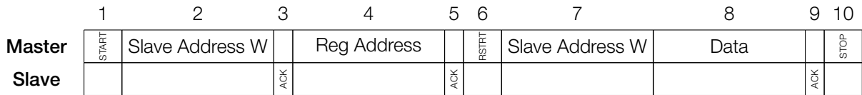
Figure 150: I2C Write Operation
