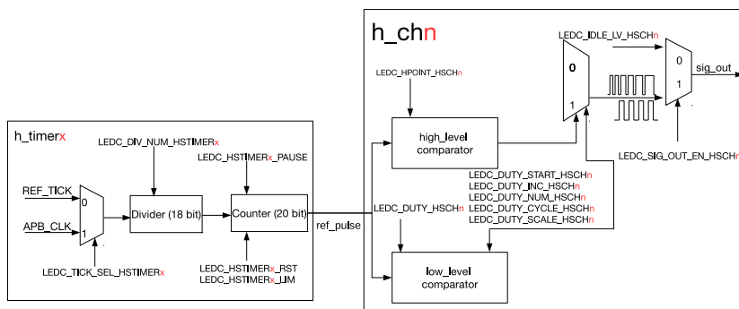
Figure 74: LED_PWM High-speed Channel Diagram
