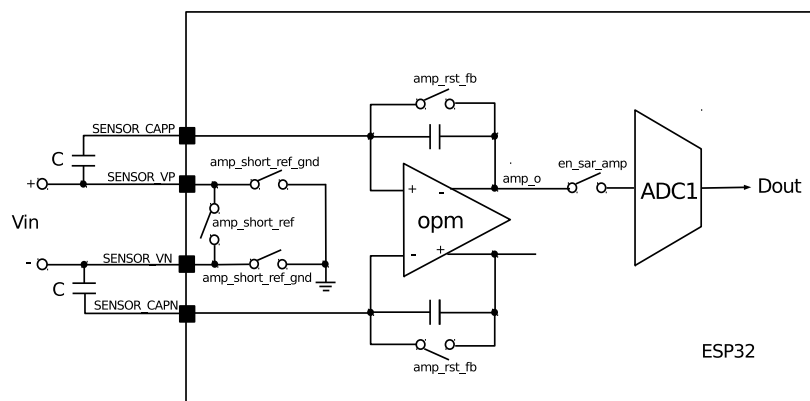
Figure 122: Structure of Low-Noise Amplifier
