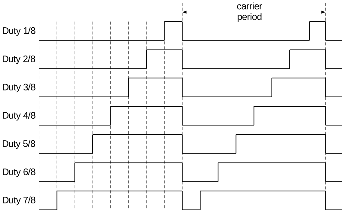
Figure 107: Possible Duty Cycle Settings for Sustaining Pulses in the PWM Carrier Submodule
