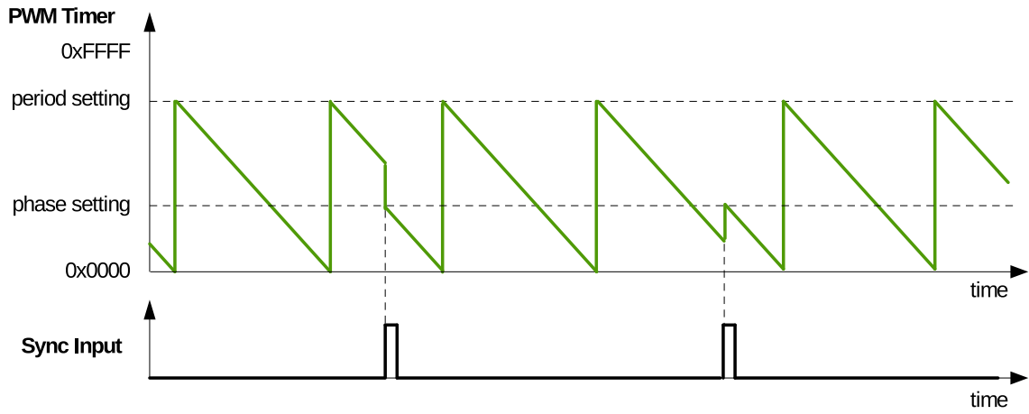
Figure 86: Count-Down Mode Waveforms
