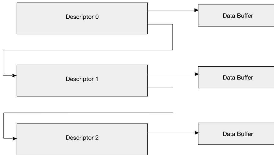
Figure 35: Descriptor Chain
