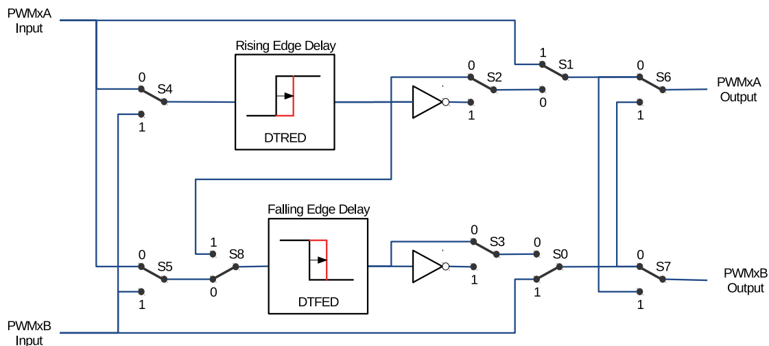
Figure 100: Options for Setting up the Dead Time Generator Submodule
