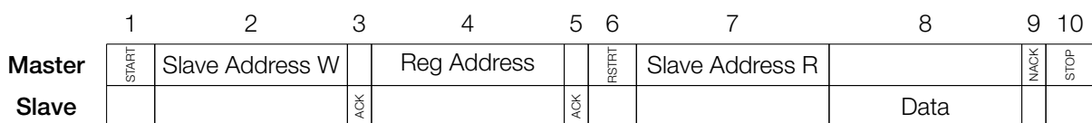
Figure 149: I2C Read Operation
