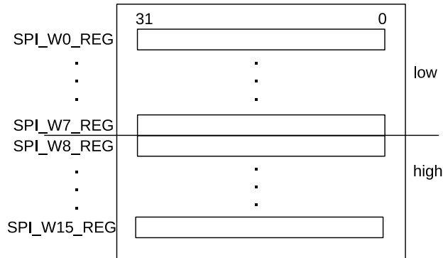
Figure 16: SPI Data Buffer
