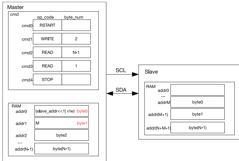
Figure 47: I2C Master Reads N Bytes of Data from addrM in Slave with 7-bit Address
