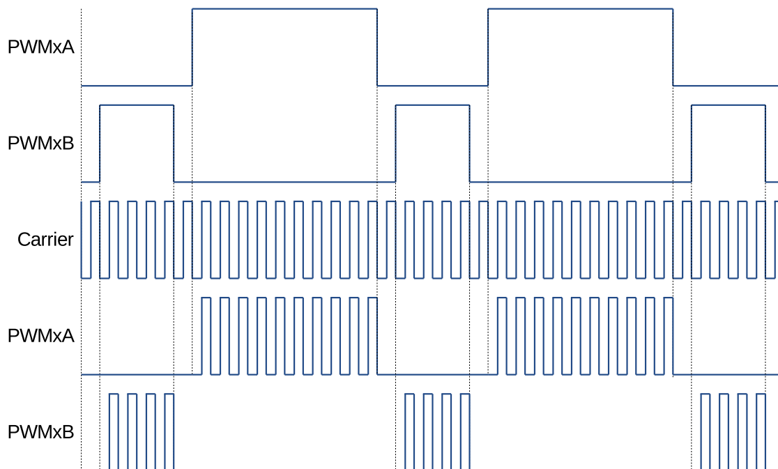
Figure 105: Example of Waveforms Showing PWM Carrier Action
