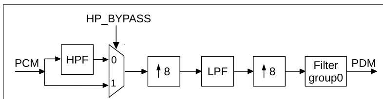
Figure 57: PDM Transmitting Module
