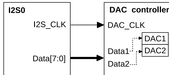
Figure 66: DAC Interface of I2S
