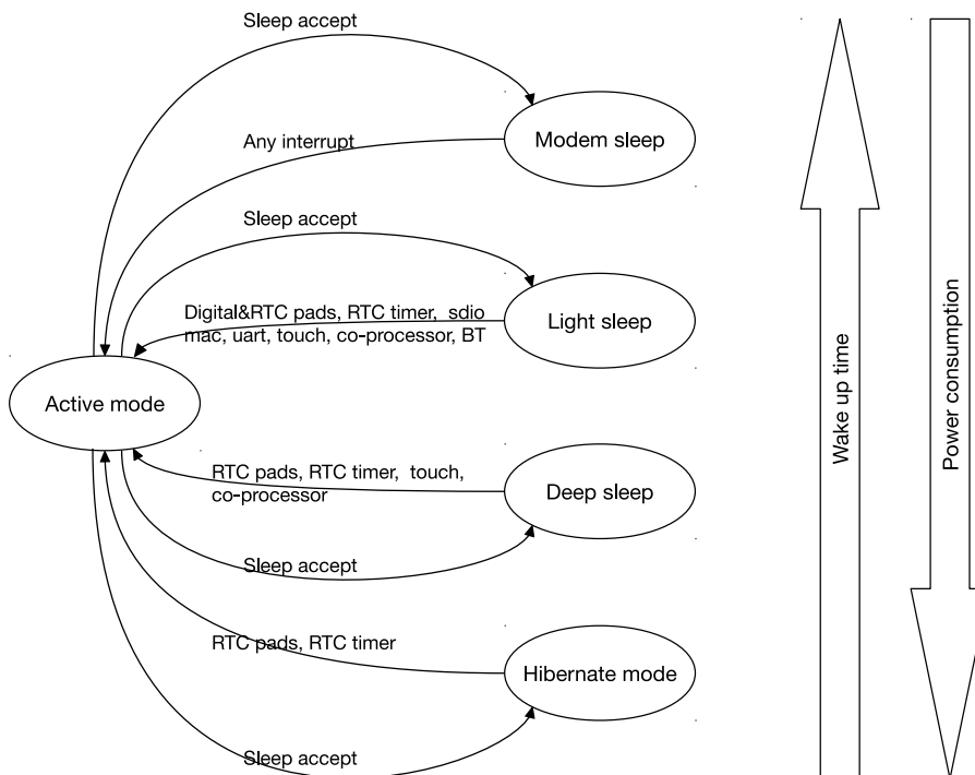
Figure 160: Power Modes
