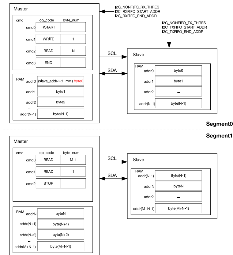
Figure 48: I2C Master Reads from Slave with 7-bit Address in Two Segments
