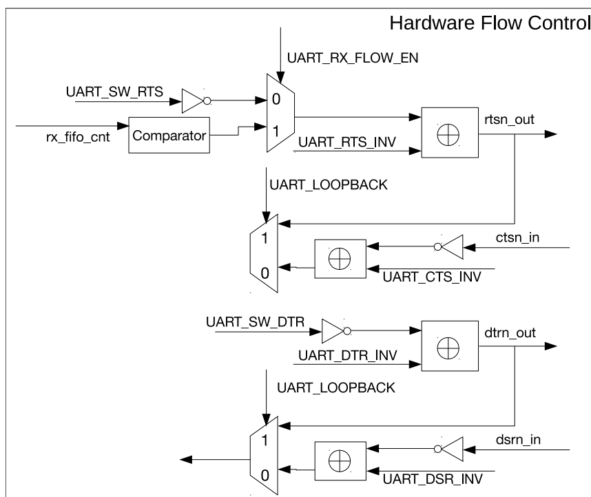
Figure 72: Hardware Flow Control
