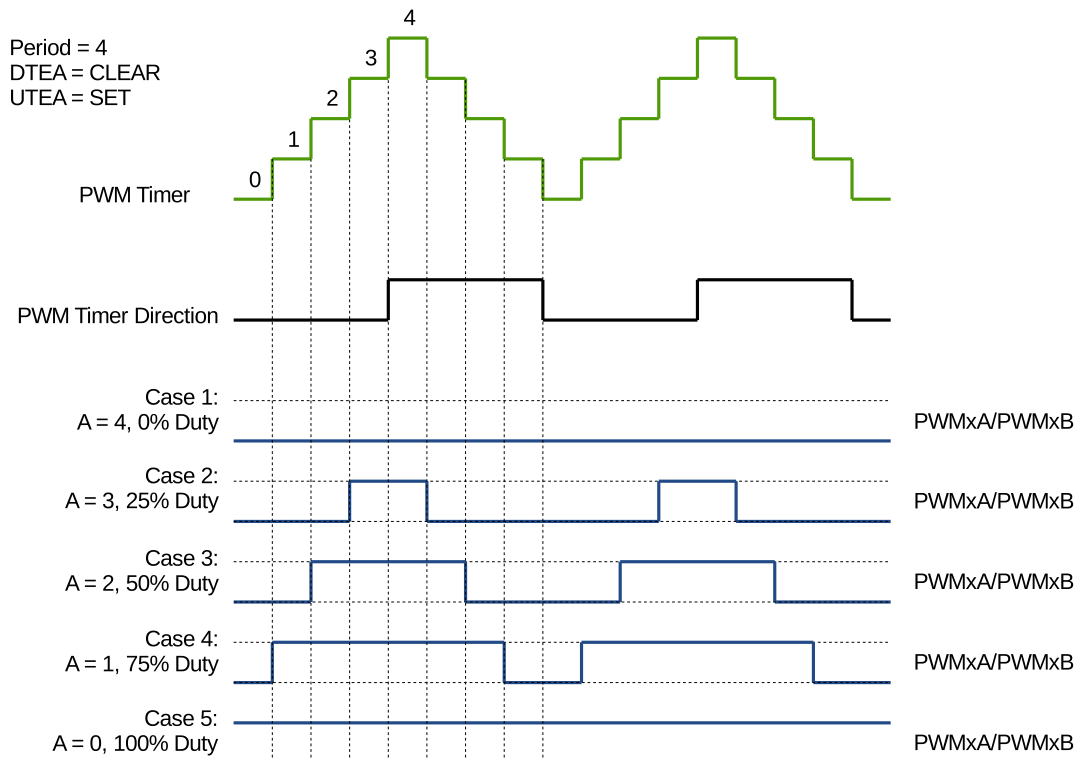
Figure 93: Symmetrical Waveform in Count-Up-Down Mode
