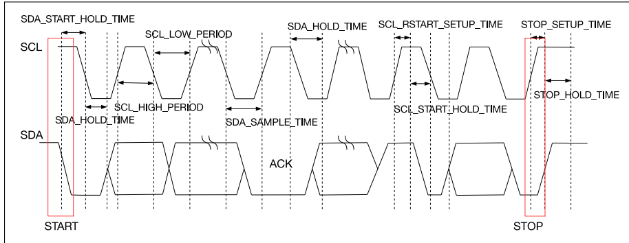
Figure 39: I2C Sequence Chart
