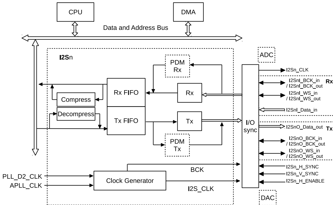
Figure 49: I2S System Block Diagram
