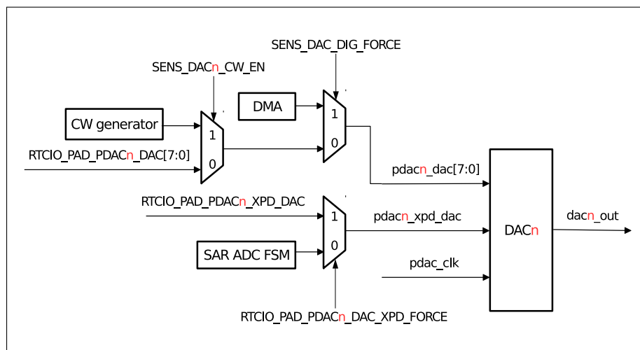
Figure 126: Diagram of DAC Function
