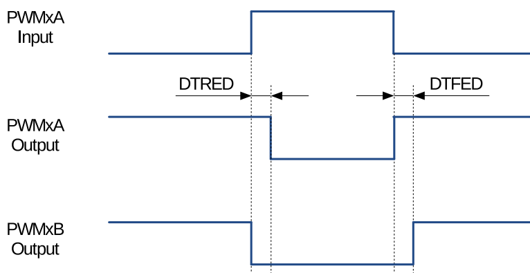
Figure 104: Active Low (AL) Dead Time Waveforms
