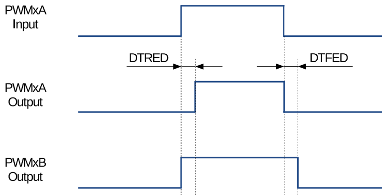
Figure 103: Active High (AH) Dead Time Waveforms
