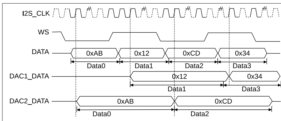
Figure 67: Data Input by I2S DAC Interface
