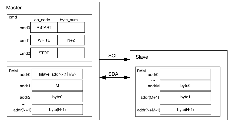
Figure 43: I2C Master Writes to addrM in RAM of Slave with 7-bit Address
