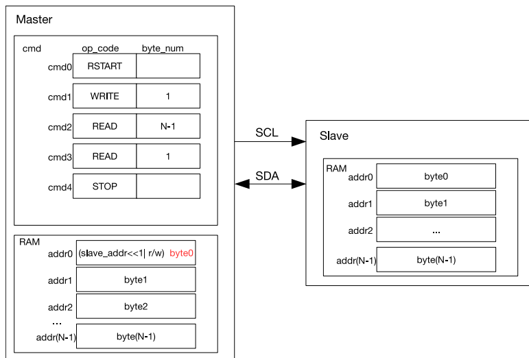
Figure 45: I2C Master Reads from Slave with 7-bit Address
