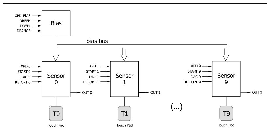
Figure 115: Touch Sensor Structure
