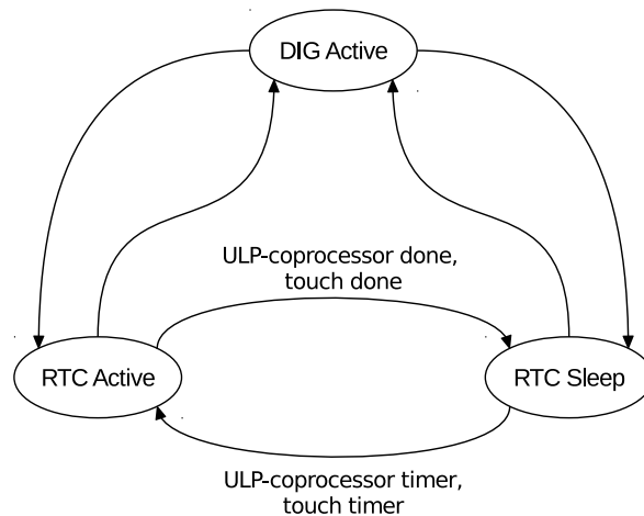
Figure 159: RTC States
