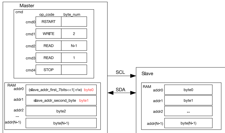
Figure 46: I2C Master Reads from Slave with 10-bit Address
