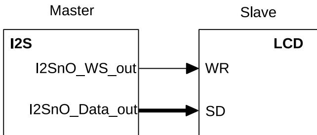
Figure 61: LCD Master Transmitting Mode
