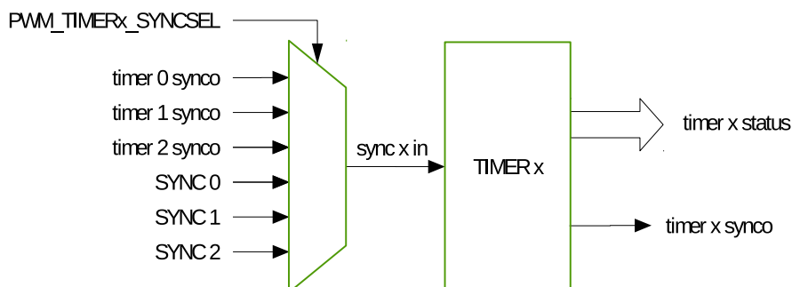
Figure 81: Timer Submodule
