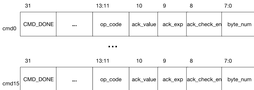
Figure 40: Structure of The I2C Command Register
