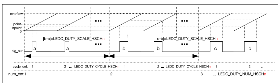
Figure 76: Output Signal Diagram of Gradient Duty Cycle
