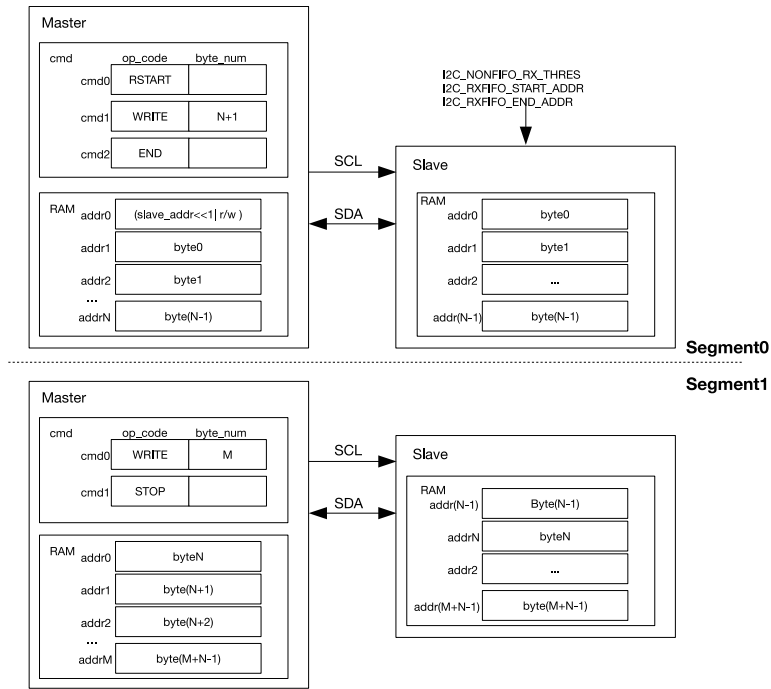
Figure 44: I2C Master Writes to Slave with 7-bit Address in Two Segments
