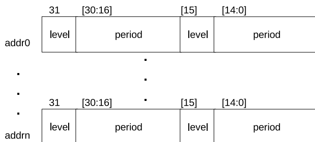
Figure 78: Data Structure
