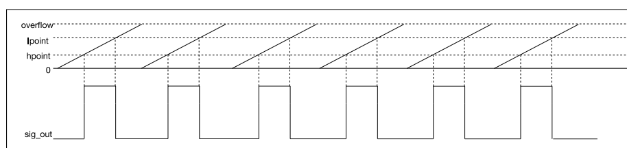
Figure 75: LED PWM Output Signal Diagram
