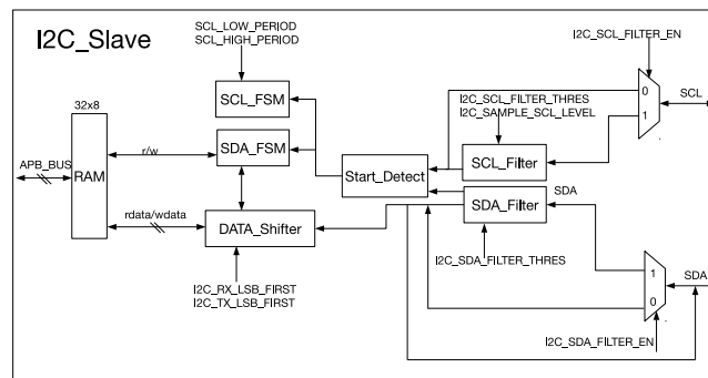
Figure 38: I2C Slave Architecture
