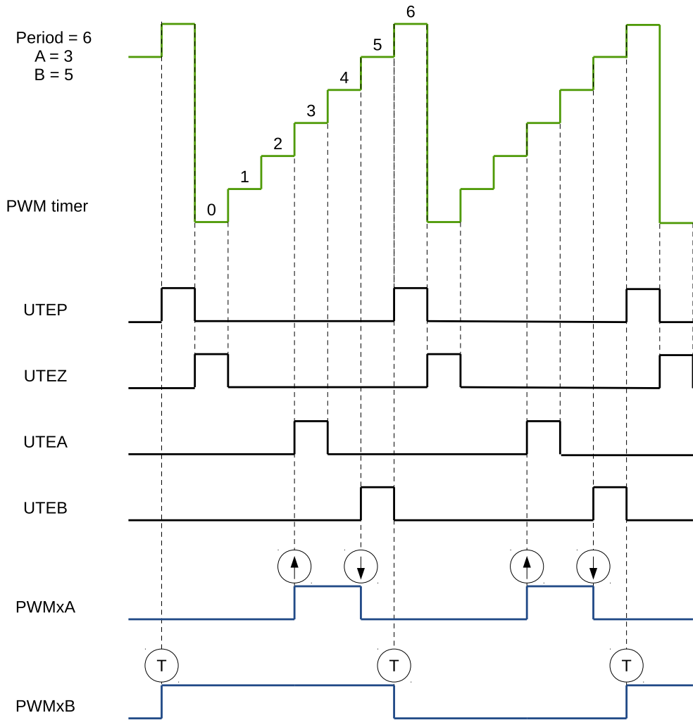
Figure 95: Count-Up, Pulse Placement Asymmetric Waveform with Independent Modulation on PWMxA
