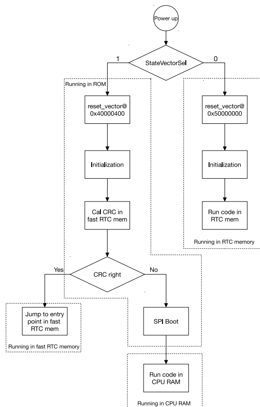
Figure 161: ESP32 Boot Flow
