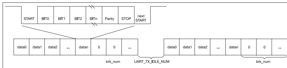
Figure 70: UART Data Frame Structure
