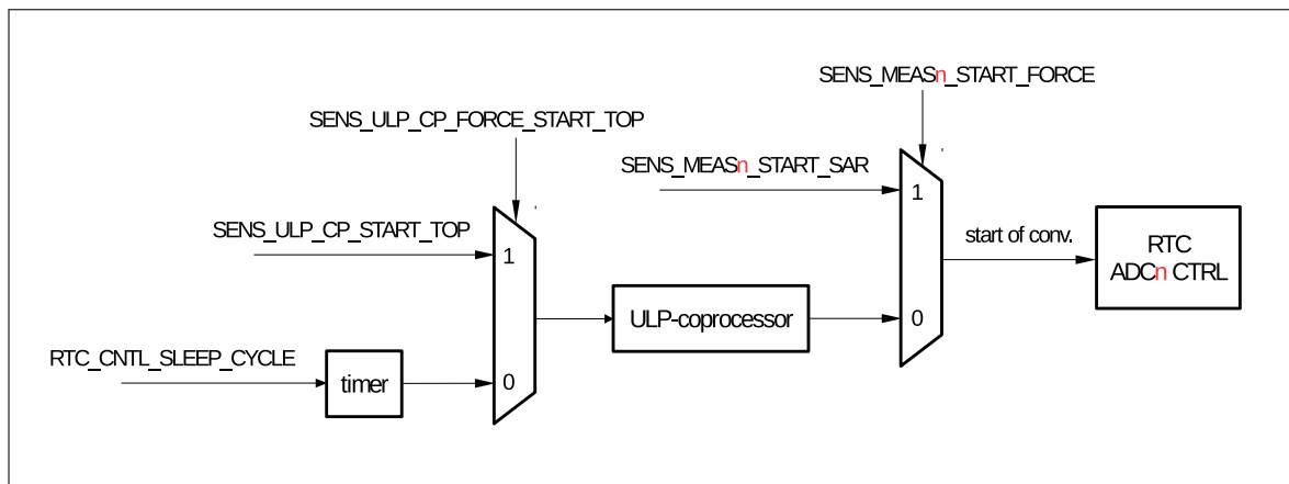
Figure 120: RTC SAR ADC Outline of Function
