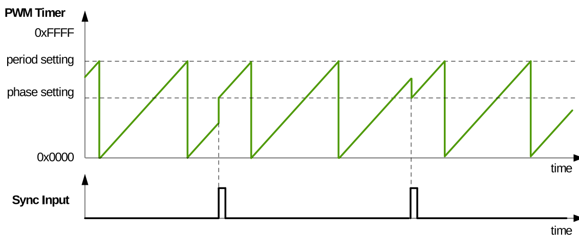
Figure 85: Count-Up Mode Waveform
