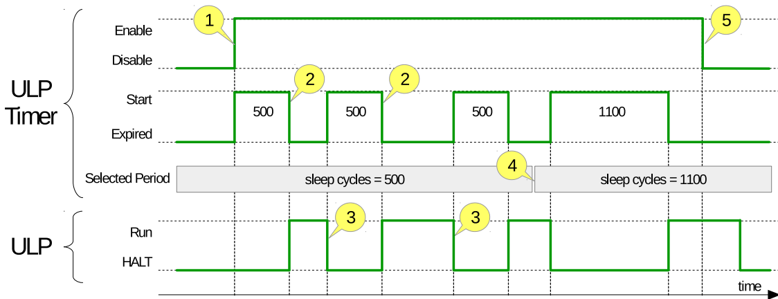
Figure 148: Sample of a ULP Operation Sequence
