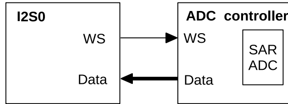
Figure 65: ADC Interface of I2S0
