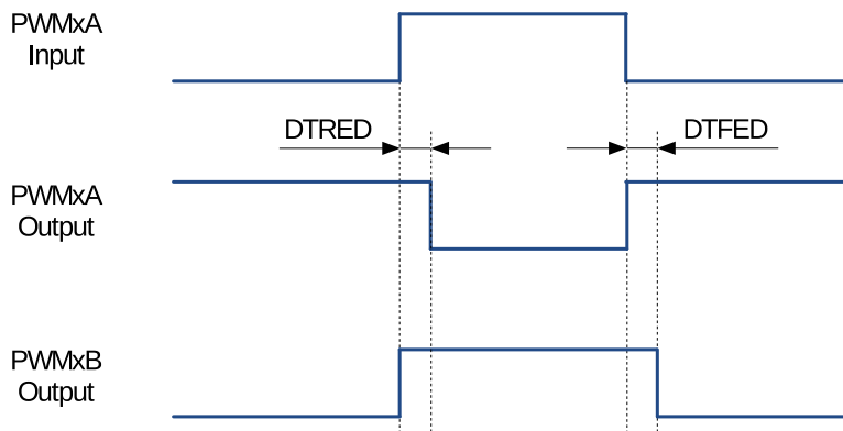
Figure 102: Active Low Complementary (ALC) Dead Time Waveforms
