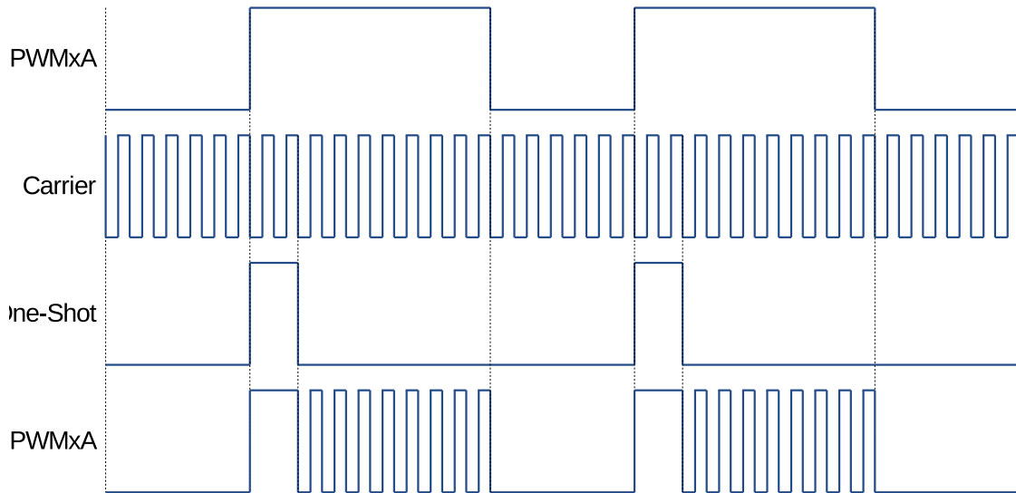
Figure 106: Example of the First Pulse and the Subsequent Sustaining Pulses of the PWM Carrier Submodule
