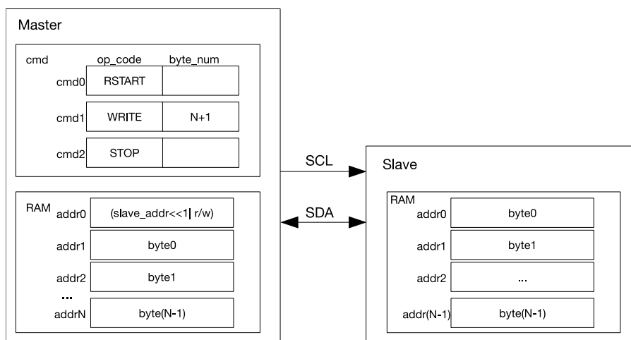
Figure 41: I2C Master Writes to Slave with 7-bit Address
