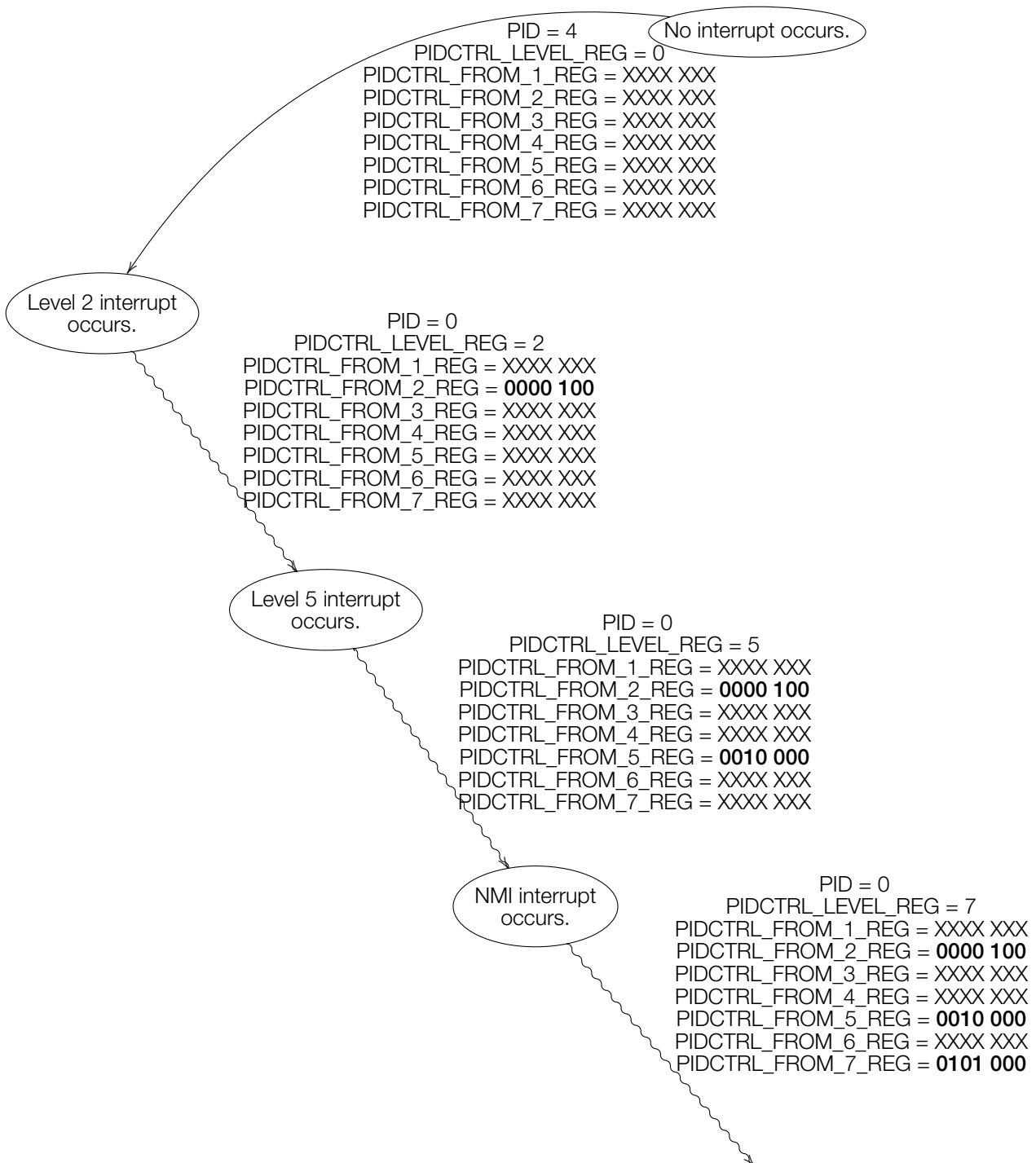
Figure 113: Interrupt Nesting
