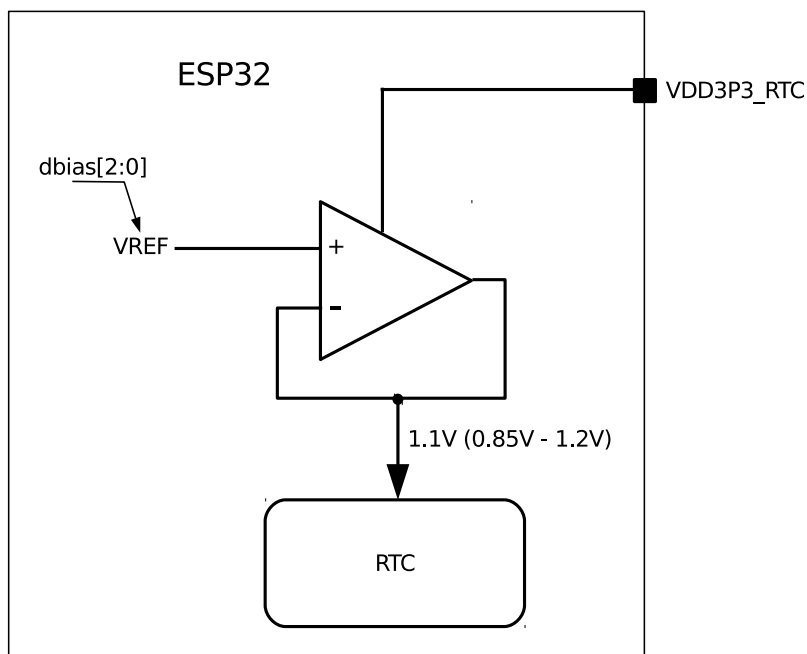
Figure 153: Low-Power Voltage Regulator
