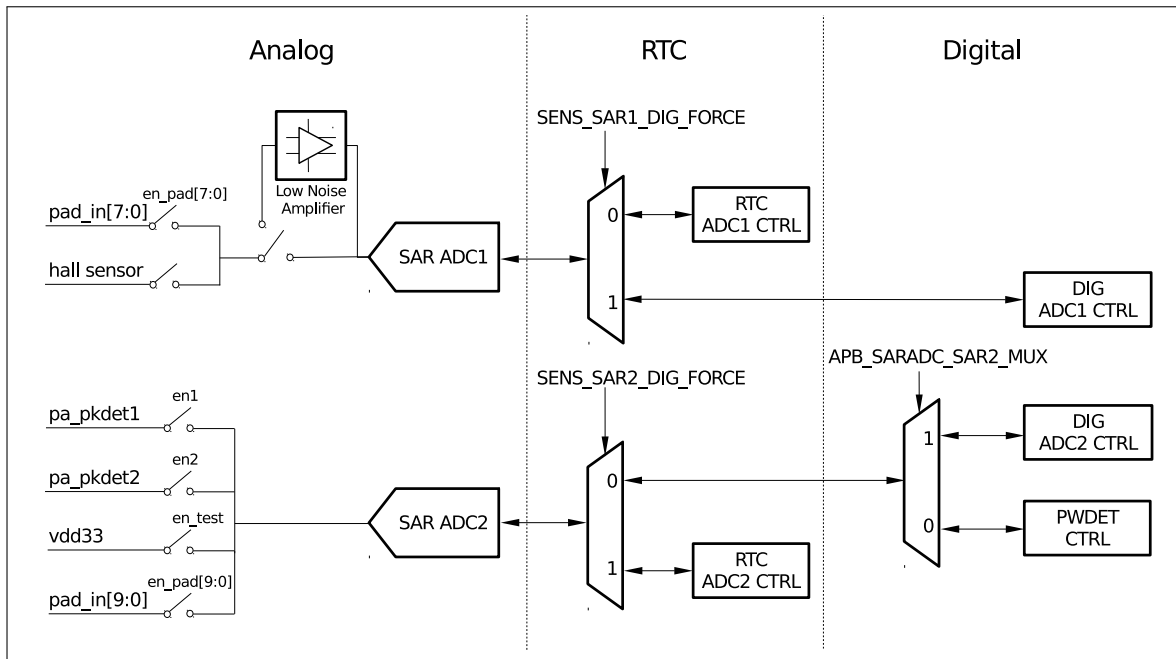
Figure 119: SAR ADC Outline of Function
