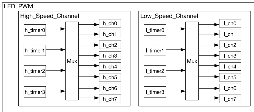
Figure 73: LED_PWM Architecture
