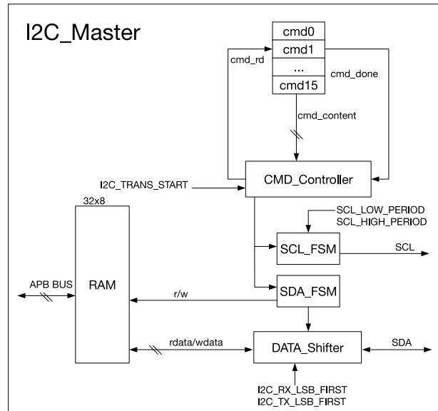
Figure 37: I2C Master Architecture
