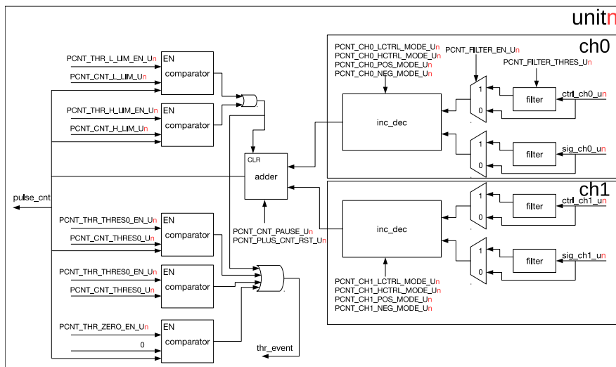
Figure 108: PULSE_CNT Architecture
